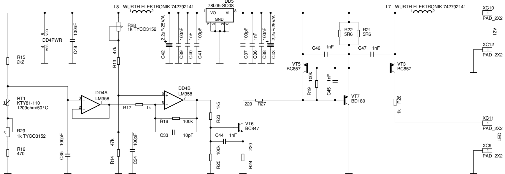
OCXO by DF9LN, modification and PCB by OK1CJH 2012
